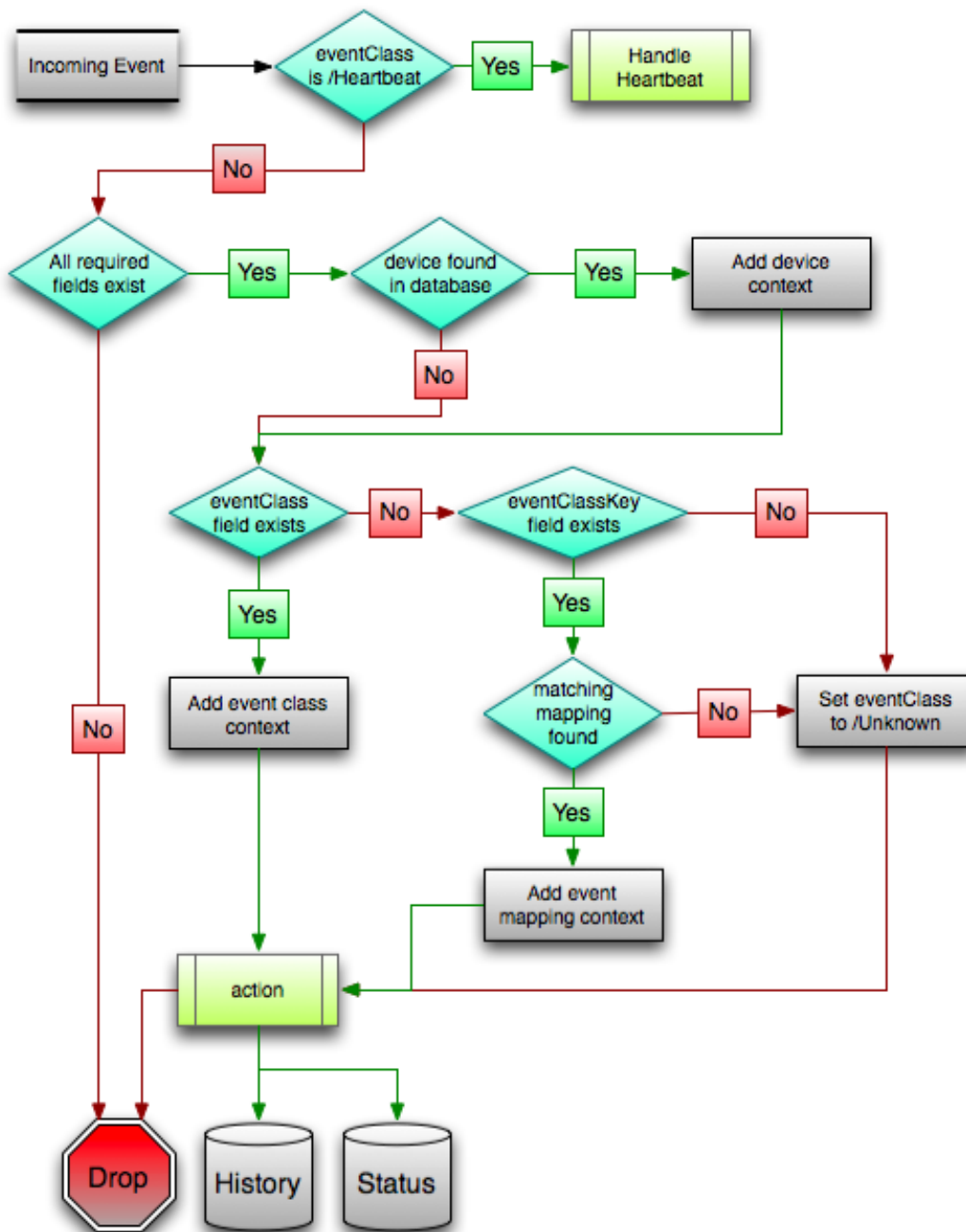
Figure 87: Event Processing
