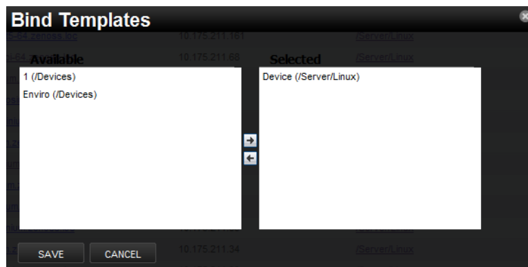
Figure 72: Bind Templates
