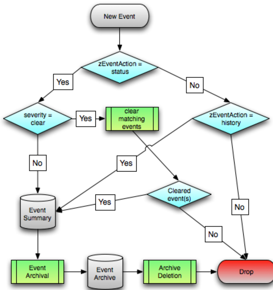
Figure 88: Event Life Cycle
