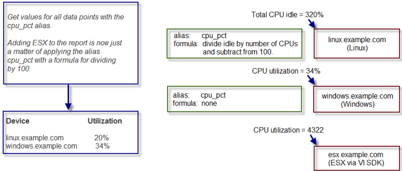
Figure 74: Alias-Based CPU Utilization Report
