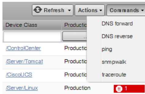
Figure 98: Run Commands
