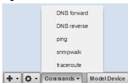
Figure 100: Commands Menu
