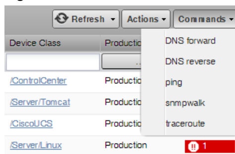
Figure 102: Run Commands
