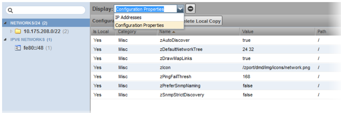
Figure 59: Networks
