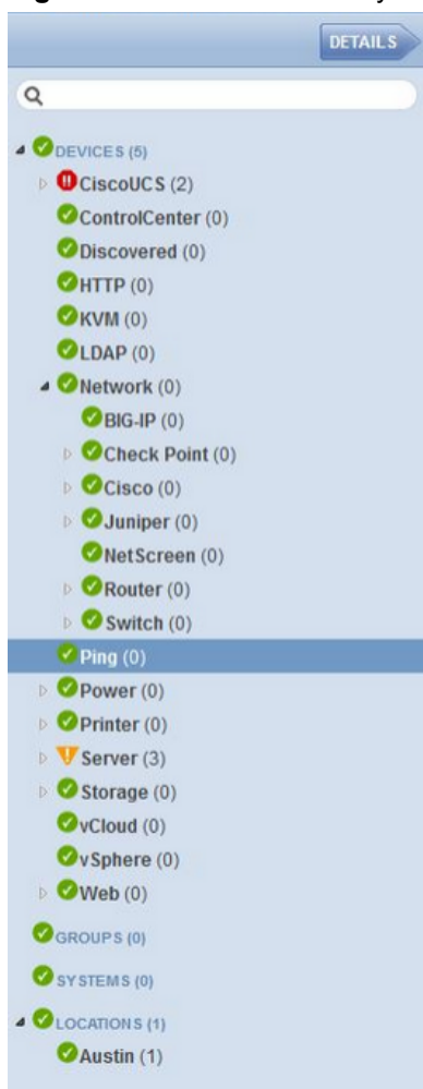
Figure 92: Devices Hierarchy
