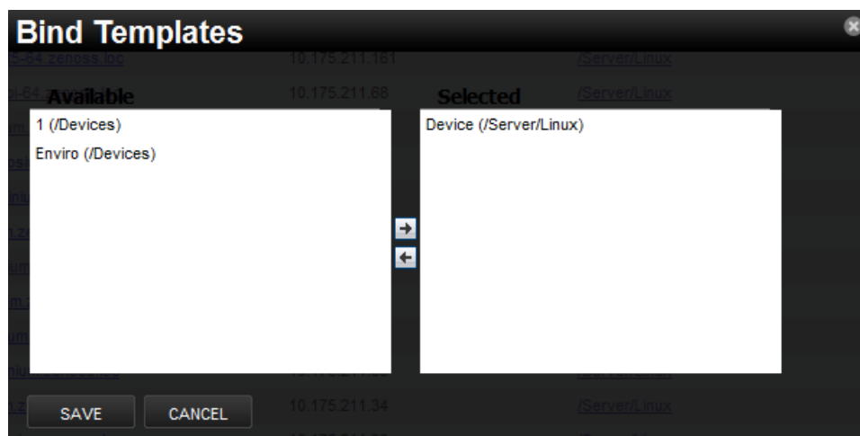
Figure 60: Bind Templates
