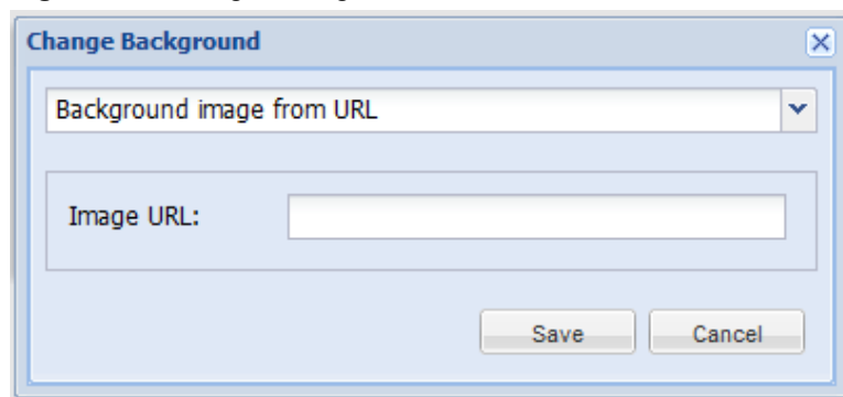
Figure 35: Change Background
