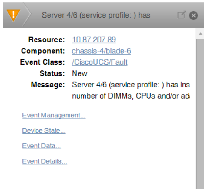
Figure 85: Event Details
