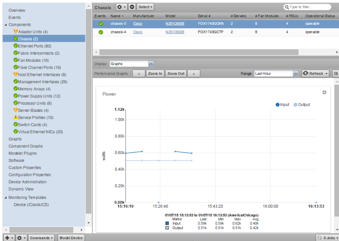
Figure 43: Device (Components)
