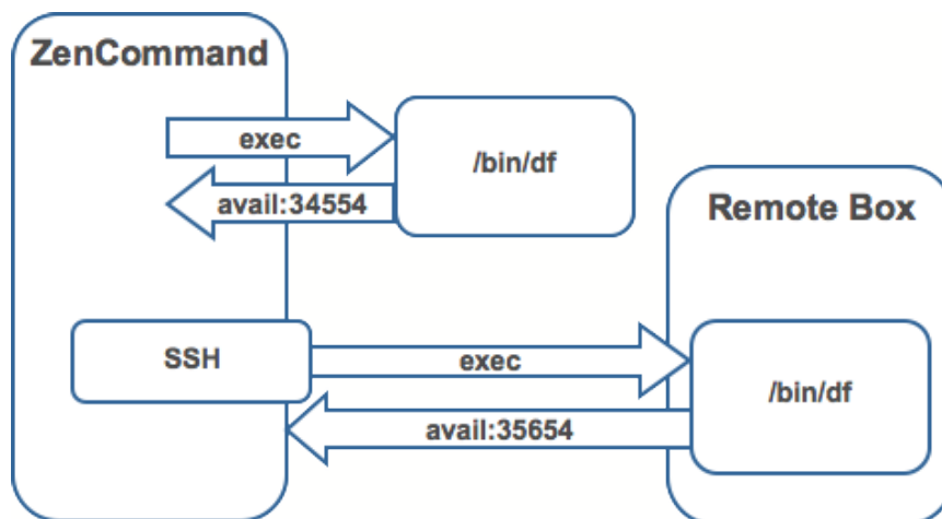
Figure 68: Running ZenCommand
