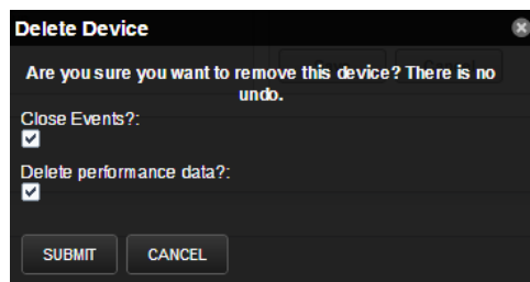
Figure 53: Delete Device
