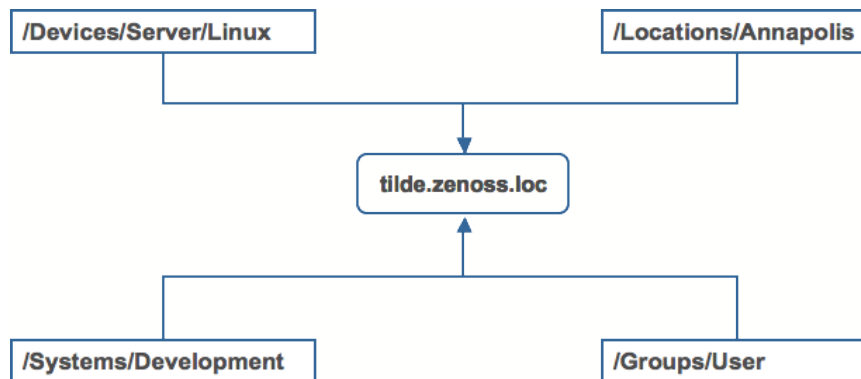
Figure 91: Device Groupings
