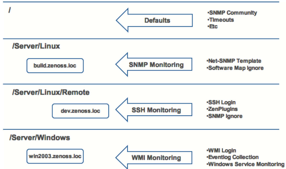
Figure 101: Device Class Tree and Inheritance
