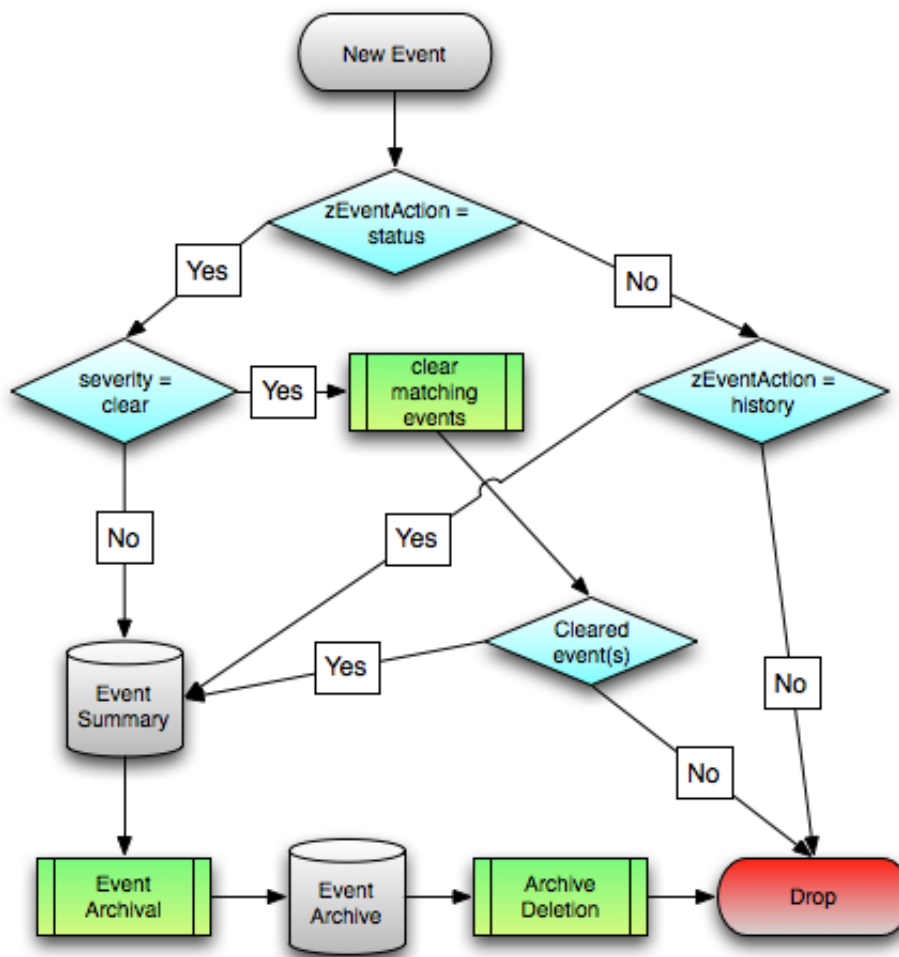
Figure 93: Event Life Cycle
