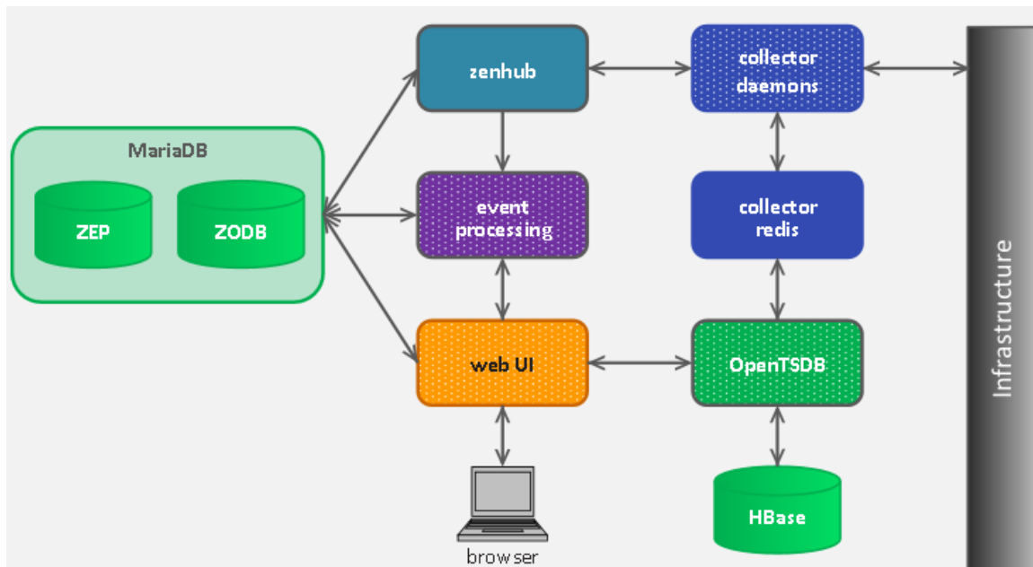
Figure 75: Data Collection Simplified Architecture
